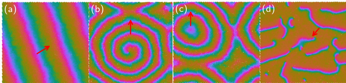
Figure 1: Waves of particle deformation spontaneously organize into various spatiotemporal patterns. Colors refer to particle sizes. Taken from [3].
