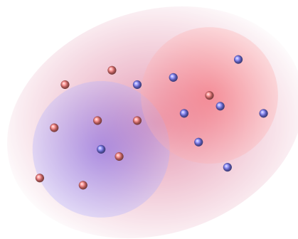
Figure 1 : A collision between a spin- \uparrow and a spin- \downarrow fermionic quasiparticle (red and blue clouds), made of fermionic particles (red and blue dots)
